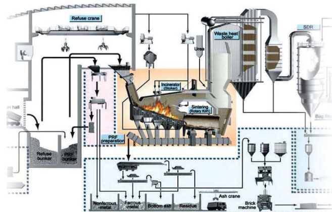
Stoker+Rotary Kiln
